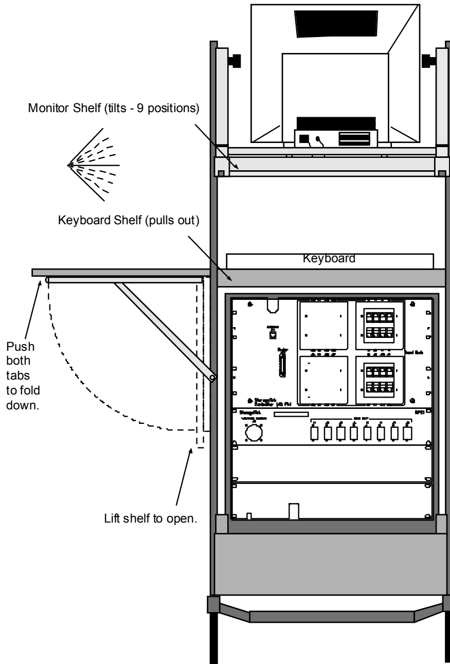
Figure 3-2. Viking CATS Rear View
