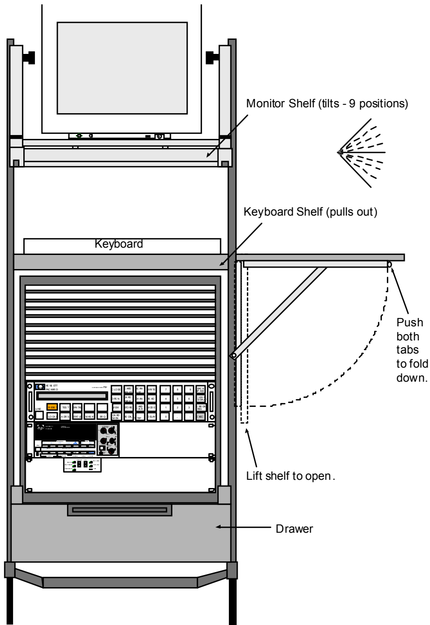
Figure 3-1. Viking CATS Front View
